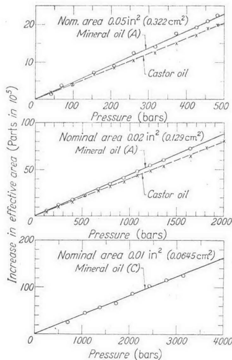
Fig. 3. Distortion factors of a group of steel piston-cylinder assemblies of type a
